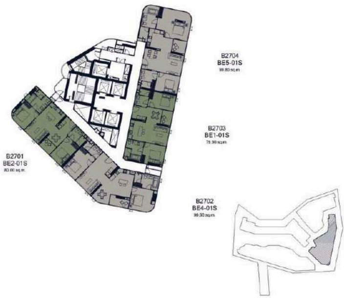
27 TH - 28 TH FLOOR PLAN
